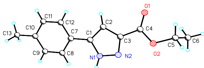
Figure 1. Crystal structure of 3b .
