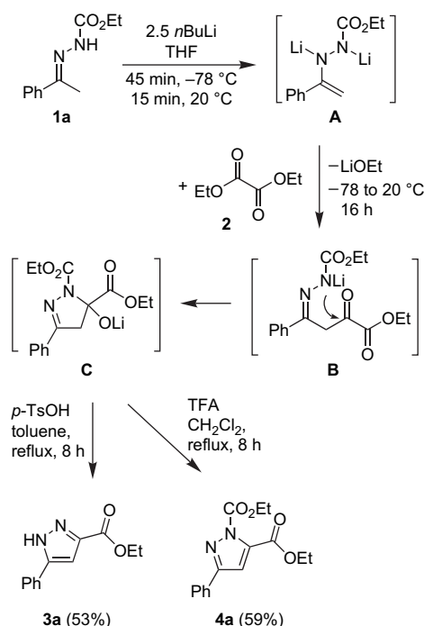
Scheme 1. Mechanism of the formation of pyrazole-3-carboxylate 3a and of pyrazole-1,5-dicarboxylate 4a .
