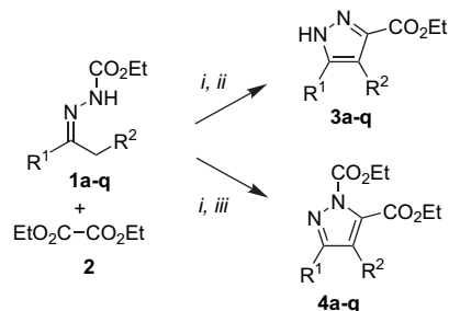
Scheme 2. Synthesis of pyrazole-3-carboxylates 3a–q and pyrazole-1,5-dicarboxylates 4a–q . (i) (1) n -BuLi (2.5 equiv), THF, 45 min, -78 °C; (2) 15 min, 20 °C; (3) 2 , -78 \rightarrow 20 °C, 16 h; (4) removal of THF; (ii) p -TsOH (4.0 equiv), toluene, reflux, 8 h; (iii) TFA, \text{CH}_2\text{Cl}_2 , reflux, 8 h.
